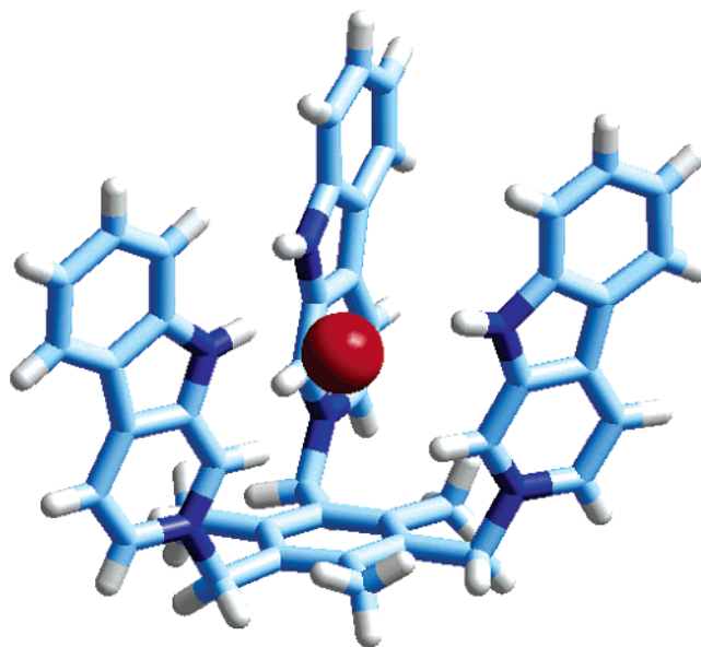
FIGURE 4. Structure of the [LH 3 ...Br] 2+ complex ([LH 3 3+ = [2] 3+ ). The complex is a part of a dimeric capsule, which consists also of a doubly deprotonated subunit including a water molecule, [LH...H 2 O] + . 10
