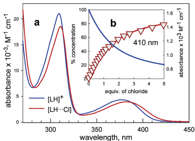
FIGURE 1. (a) Blue line, spectrum of an MeCN solution of [1]PF_6 ( 6.2 \times 10^{-4} M); red line, spectrum of the same solution + 4 equiv of [Bu_3BzN]Cl . (b) Symbols: molar absorbance at 410 nm (right side vertical axis) vs equiv of Cl^- . Lines: % concentration (left side vertical axis); blue line, receptor [1]^+ ; and red line, chloride complex, [1 \cdots Cl] .
