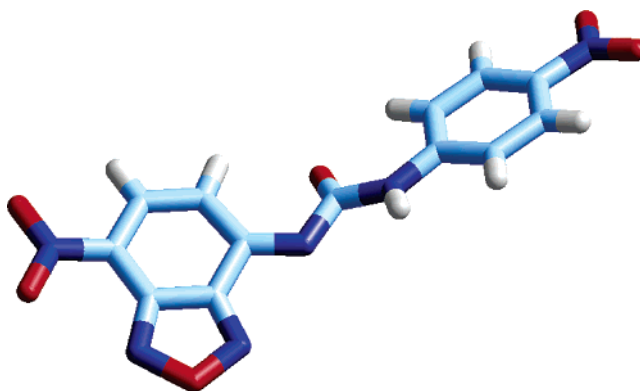
FIGURE 12. Structure of the \text{L}^- anion (LH = 5 ). The tetrabutylammonium counteraction has been omitted. 20
